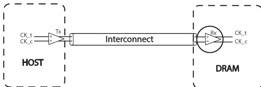
Figure 14. HOST driving clock signals to the DRAM
