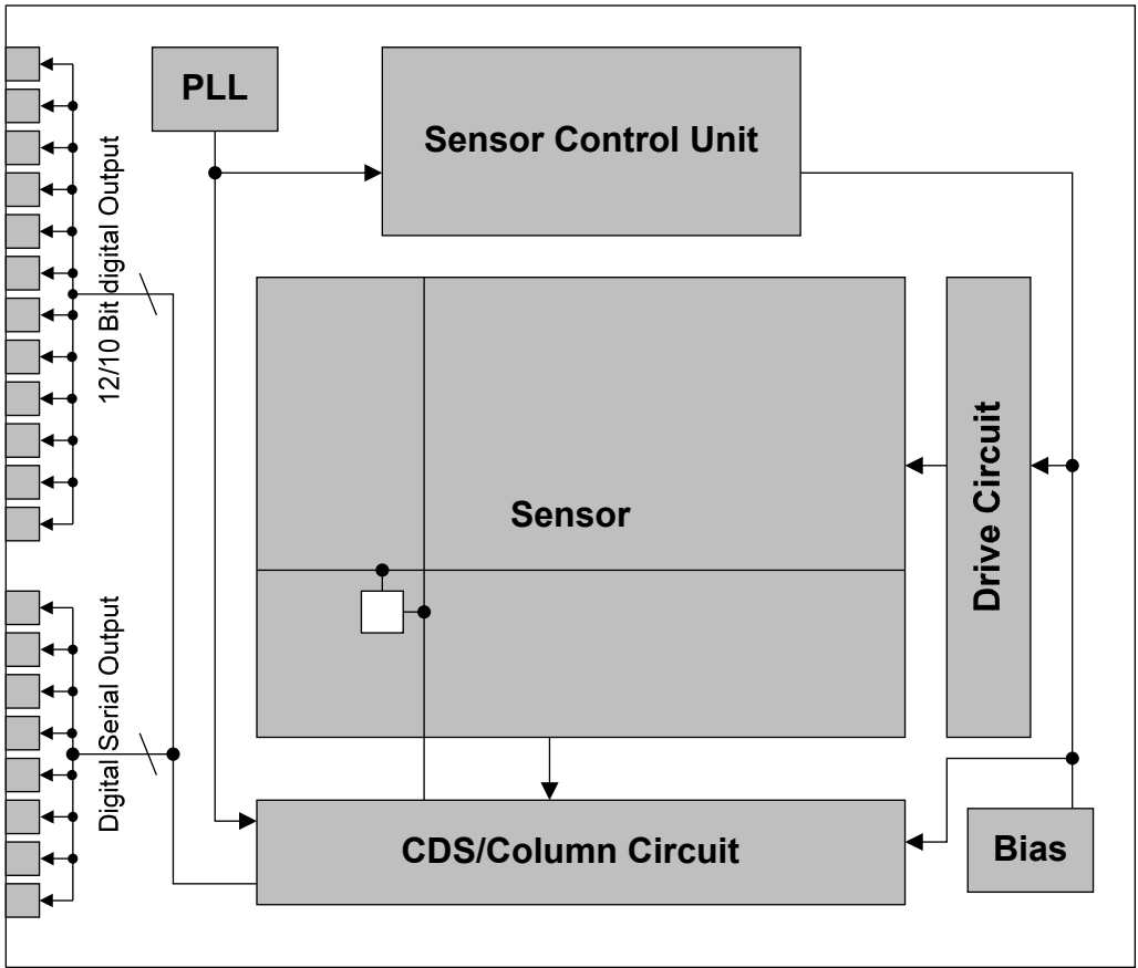
Block Diagram
