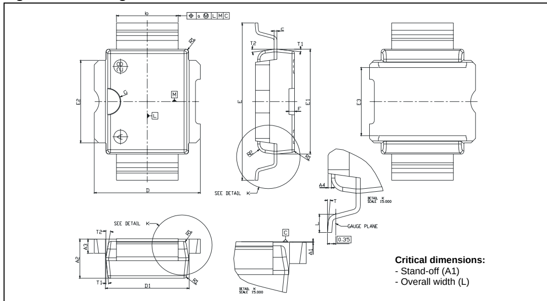
Figure 34. Package dimensions
