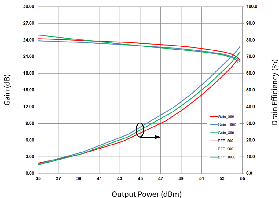
Figure 3. Gain and Drain Efficiency vs. Frequency and Output Power CGHV40180F-TB CW Operation, V_{DD} = 50 V, I_{DQ} = 1.0 A
