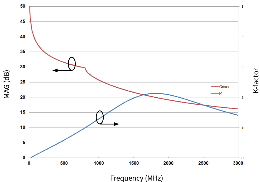
Figure 4. Simulated Maximum Available Gain and K-factor of the CGHV40180F V_{DD} = 50 V, I_{DQ} = 1.0 A
