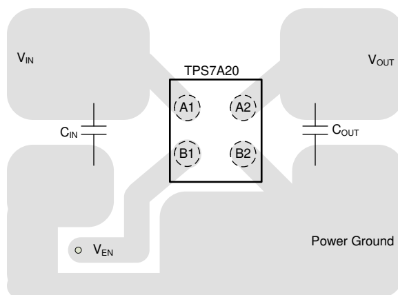
图 7-9. YCJ and YCK Package (DSBGA) Typical Layout
