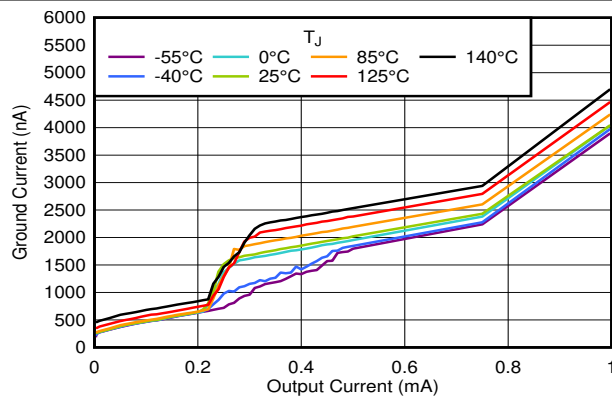
图 6-5. I_Q vs I_{OUT} and Temperature Up to 1 mA
