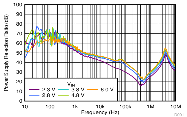
V_{OUT} = 1.8\text{ V} , I_{OUT} = 100\text{ mA} , C_{OUT} = 1\text{ }\mu\text{F} 图 6-46. PSRR vs Frequency and V_{OUT}
