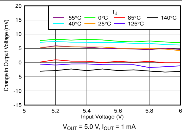
图 6-28. Line Regulation vs V_{IN} and Temperature
