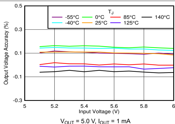
图 6-29. Output Accuracy vs V_{IN} and Temperature
