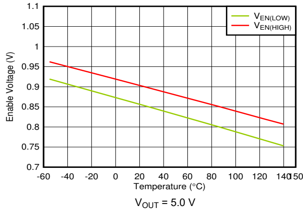
图 6-39. EN High and Low Threshold vs Temperature
