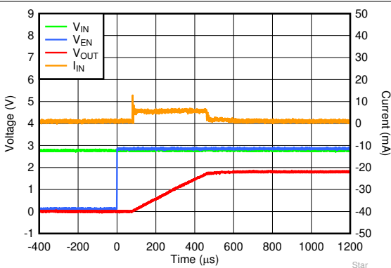
图 6-55. Startup Inrush Current With C_{OUT} = 1\text{ }\mu\text{F}
