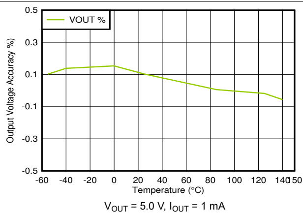
图 6-30. Output Accuracy vs Temperature
