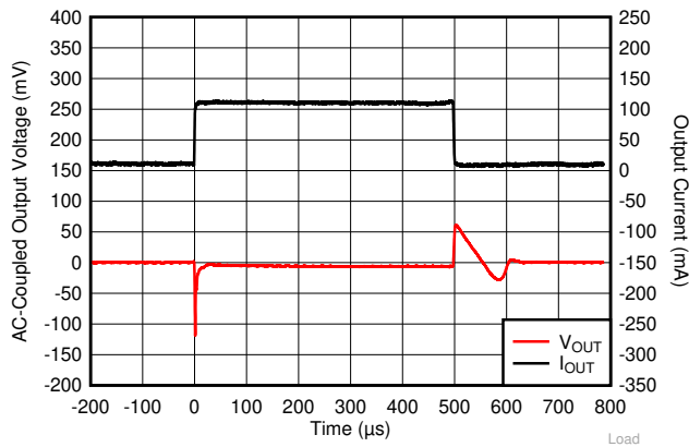
图 6-13. I_{OUT} Transient From 1 mA to 100 mA
