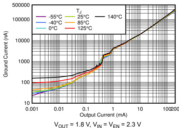
图 6-3. I_Q vs I_{OUT} and Temperature up to 200 mA
