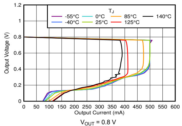
图 6-36. Foldback Current Limit vs I_{OUT} and Temperature
