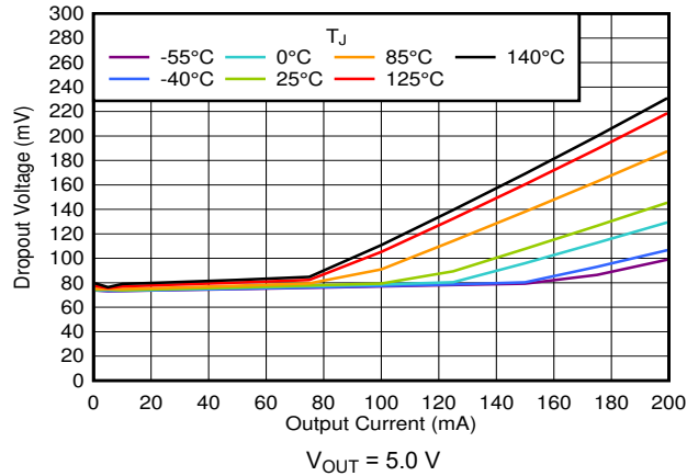
图 6-33. Dropout vs I_{OUT} and Temperature
