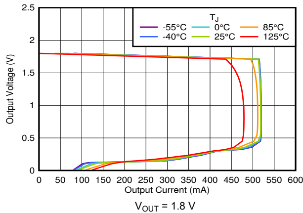
图 6-37. Foldback Current Limit vs I_{OUT} and Temperature
