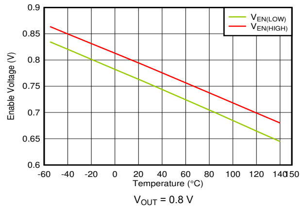
图 6-38. EN High and Low Threshold vs Temperature
