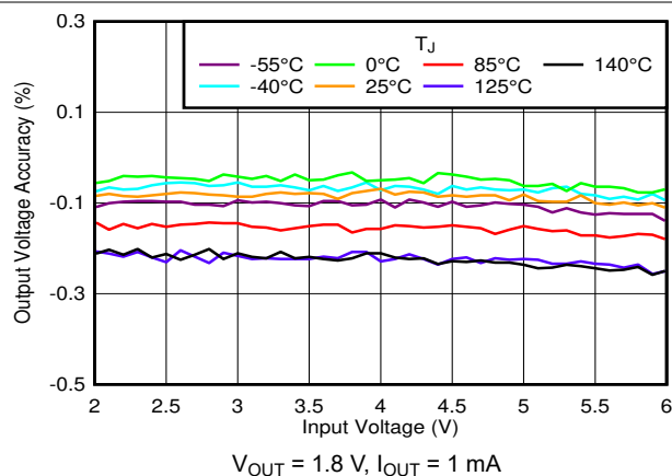
图 6-26. Output Accuracy vs V_{IN} and Temperature
