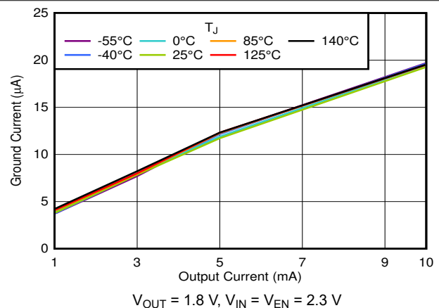
图 6-6. I_Q vs I_{OUT} and Temperature for 1 mA to 10 mA
