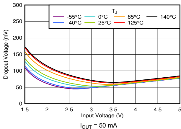
图 6-35. Dropout vs V_{IN} and Temperature
