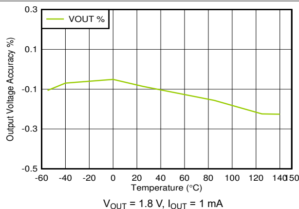
图 6-27. Output Accuracy vs Temperature
