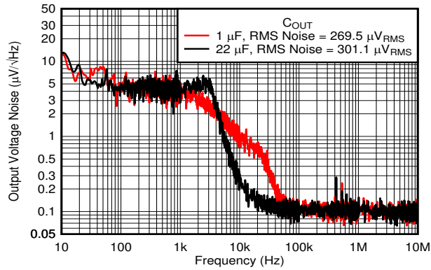
图 6-49. Output Noise vs Frequency and C_{OUT}
