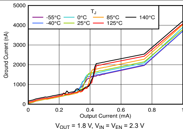
图 6-5. I_Q vs I_{OUT} and Temperature Up to 1 mA
