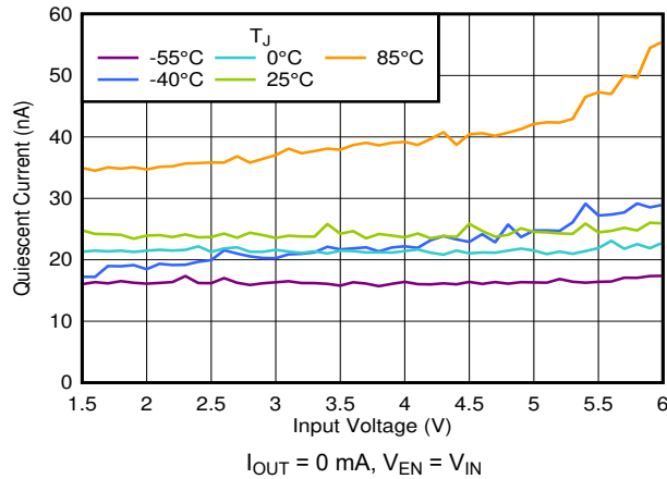
图 6-1. I_Q vs V_{IN} and Temperature
