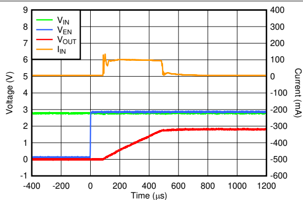
图 6-56. Startup Inrush Current With C_{OUT} = 22\text{ }\mu\text{F}
