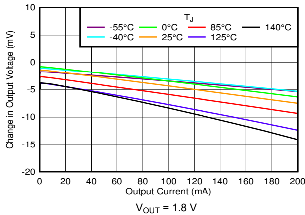
图 6-31. Load Regulation vs V_{IN} and Temperature
