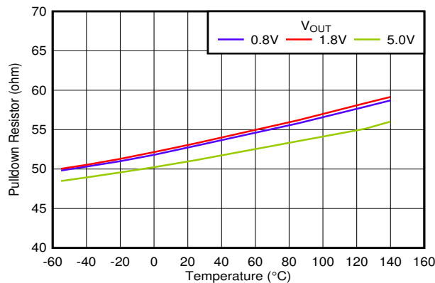
图 6-41. Pulldown Resistor vs Temperature and V_{OUT}
