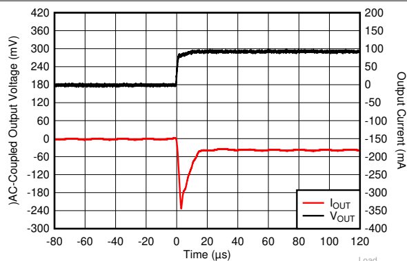
图 6-15. I_{OUT} Transient From 0 mA to 50 mA
