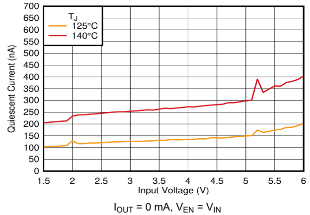
图 6-2. I_Q vs V_{IN} and Temperature
