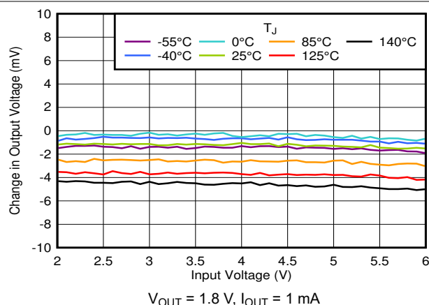
图 6-25. Line Regulation vs V_{IN} and Temperature
