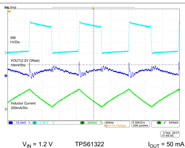
图 8-3. Switching Waveform at Heavy Load
