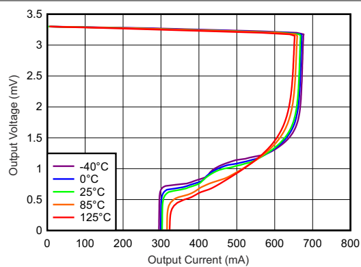
图 5-26. 3.3V Foldback Current Limit, V_{OUT} vs I_{OUT}
