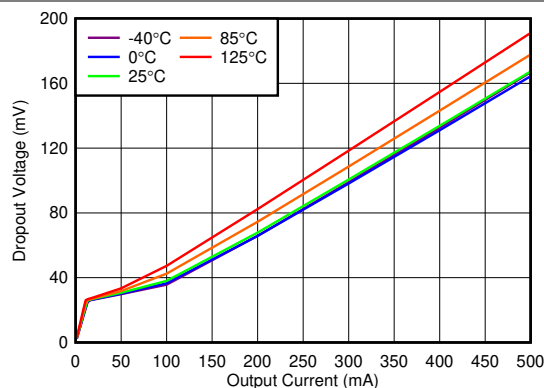
图 5-14. 5.0V Dropout Voltage vs I_{OUT}
