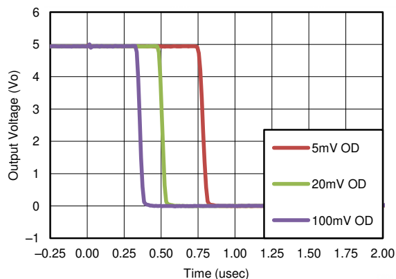
图 7-3. Response Time for Various Overdrives (Negative Transition)
