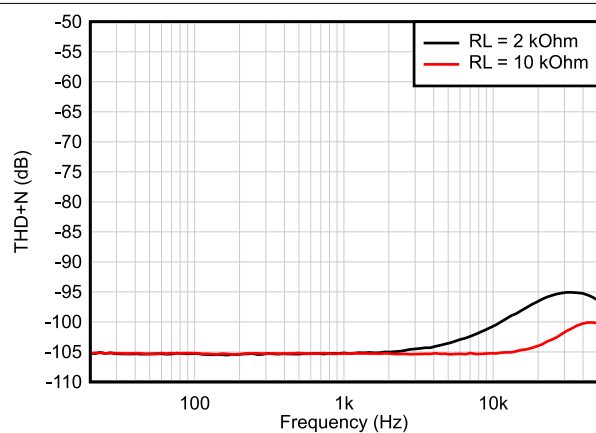
图 5-19. THD+N Ratio vs Frequency
