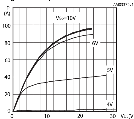
Figure 6: Output characteristics
