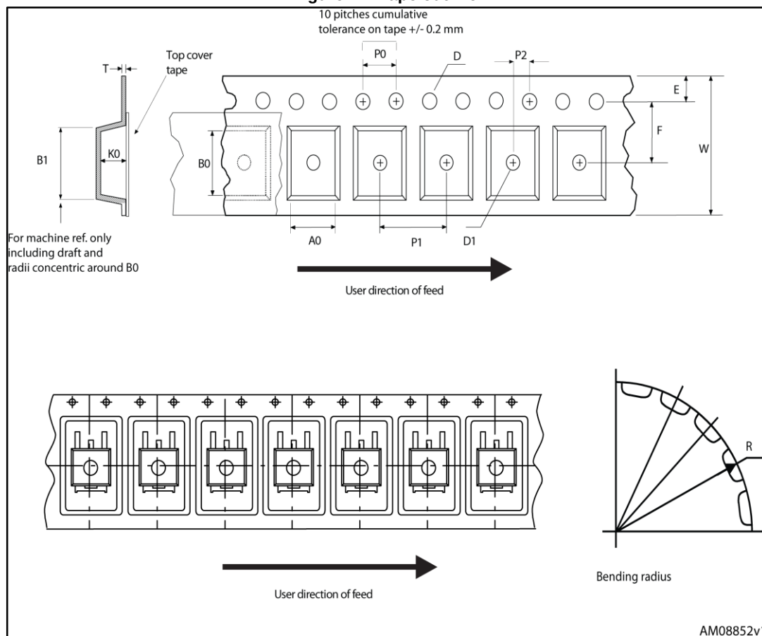
Figure 24: Tape outline
