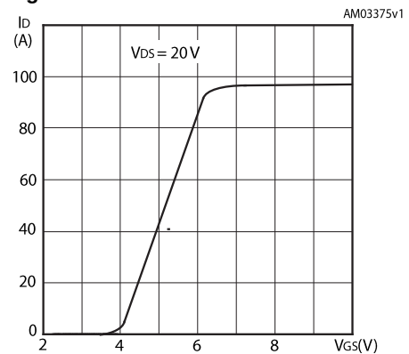
Figure 7: Transfer characteristics
