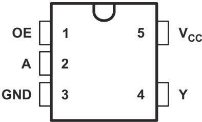
图 5-1. DCK or DBV Package, 5-Pin SC70 or SOT-23 (Top View)
