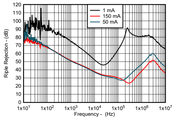
图 5-15. Ripple Rejection vs Frequency (Legacy Chip)
