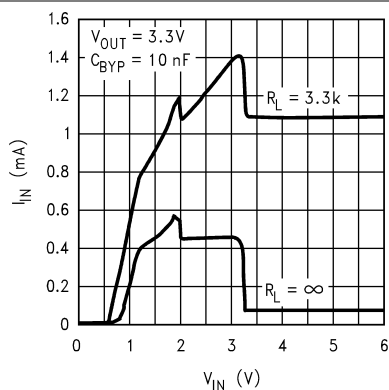
图 5-31. Input Current vs Input Voltage (Legacy Chip)
