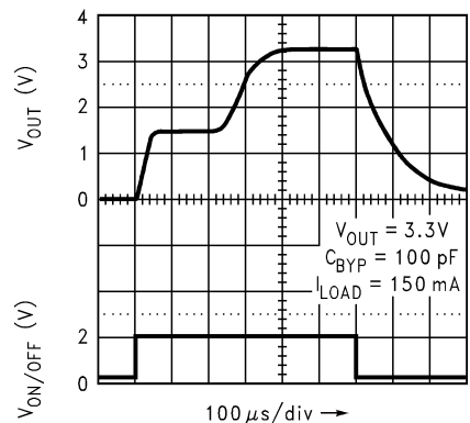
图 8-21. Turn-On Time for Legacy Chip
