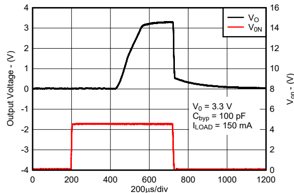
图 8-22. Turn-On Time for New Chip
