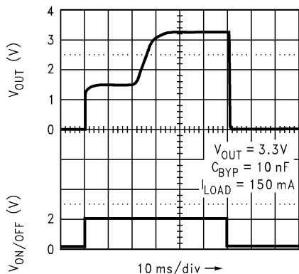
图 8-25. Turn-On Time for Legacy Chip
