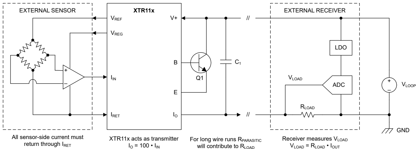
图 7-1. Typical Schematic
