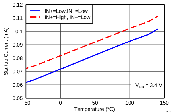
图 5. Startup Current vs Temperature
