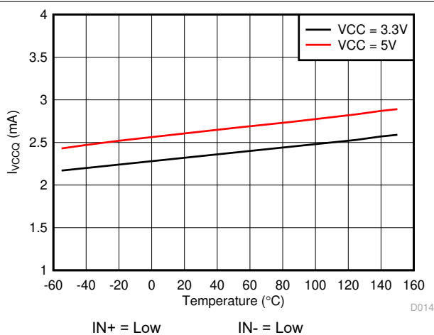
图 5-7. I_{VCCQ} Supply Current vs. Temperature
