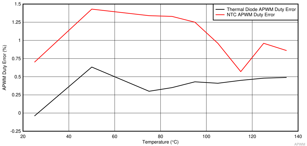
图 8-13. APWM Duty Error Without Calibration
