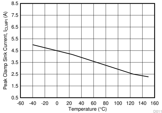
图 5-22. I_{CLMPI} Miller Clamp Sink Current vs. Temperature
