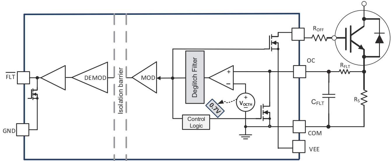
图 8-9. Overcurrent and Short Circuit Protection Based on Shunt Resistor
