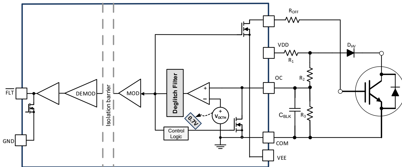
图 8-8. Overcurrent and Short Circuit Protection Based on Desaturation Circuit
