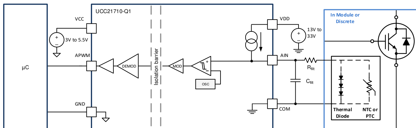
图 8-10. Thermal Diode or Thermistor Temperature Sensing Configuration
