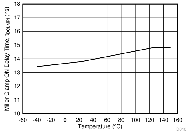
图 5-23. t_{DCLMPI} Miller Clamp ON Delay Time vs. Temperature
