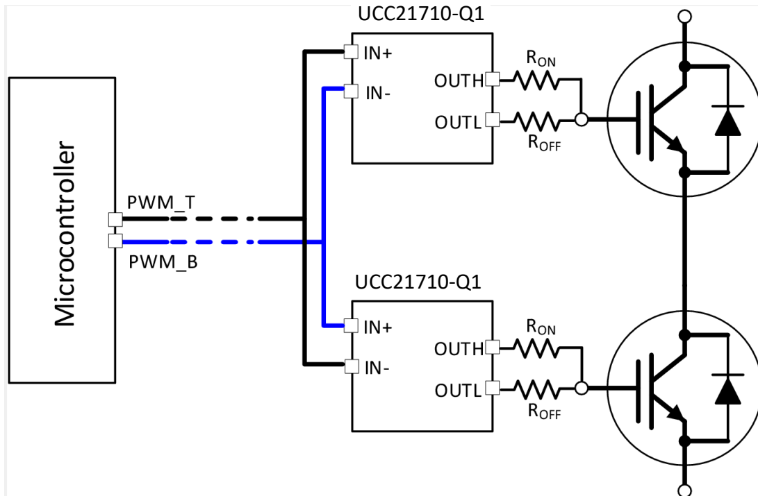
图 8-2. PWM Interlock for a Half Bridge
