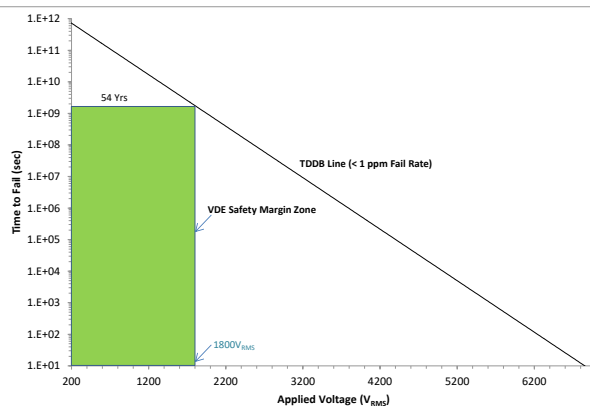
图 5-3. Reinforced Isolation Capacitor Life Time Projection
