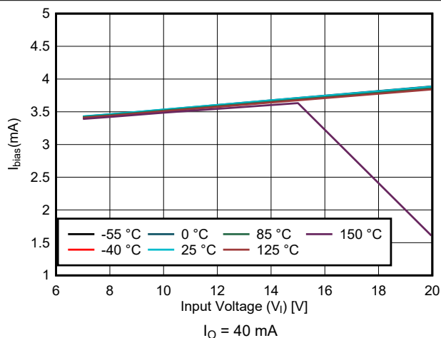
图 6-16. Bias Current vs Input Voltage for New Chip
