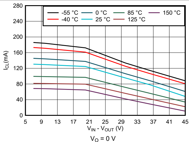
图 6-18. I_{SC} vs V_I for New Chip
