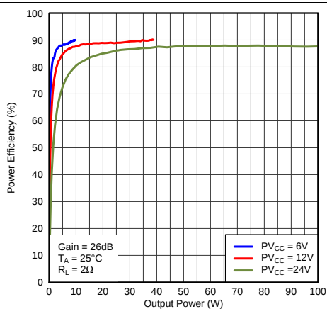
图 23. Power Efficiency (PBTL) vs Output Power
