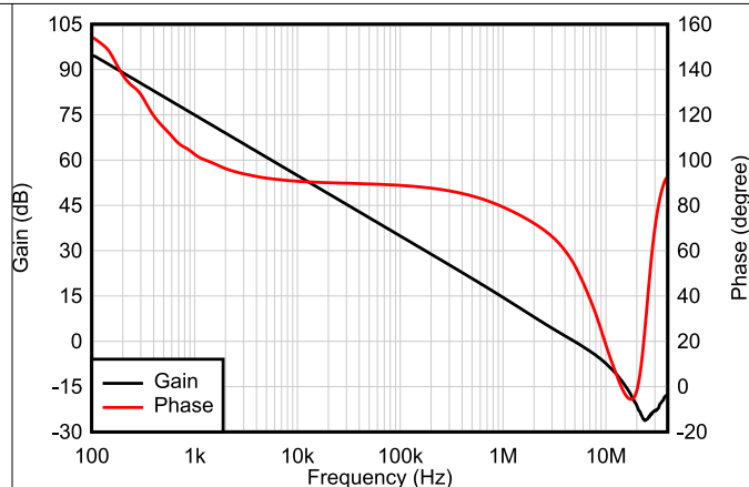
图 5-8. Open-Loop Gain and Phase vs Frequency
