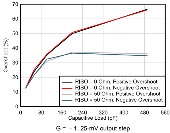
图 5-25. Small-Signal Overshoot vs Capacitive Load
