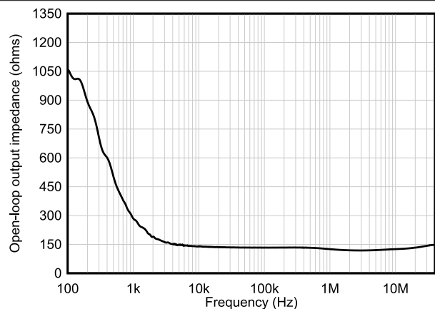
图 5-24. Open-Loop Output Impedance vs Frequency
