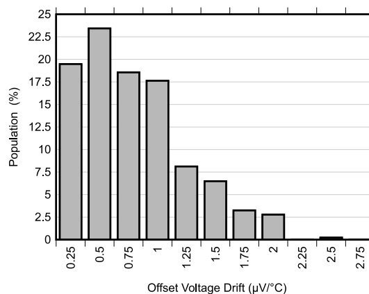
图 5-2. Offset Voltage Drift Distribution
