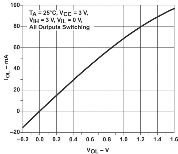
图 9-2. Output Drive Current ( I_{OL} ) vs LOW-level Output Voltage ( V_{OL} )
