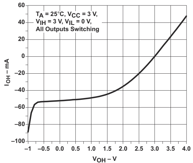
图 9-3. Output Drive Current ( I_{OH} ) vs HIGH-level Output Voltage ( V_{OH} )
