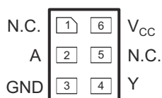
Figure 4-4. DRY Package 6-Pin SON Top View
