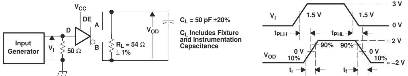
图 6-3. Test Circuit and Definitions for the Driver Common-Mode Output Voltage
