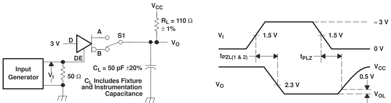
图 6-5. Driver High-Level Enable and Disable Time Test Circuit and Voltage Waveforms
