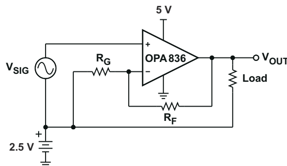
图 8-7. Single-Supply Concept
