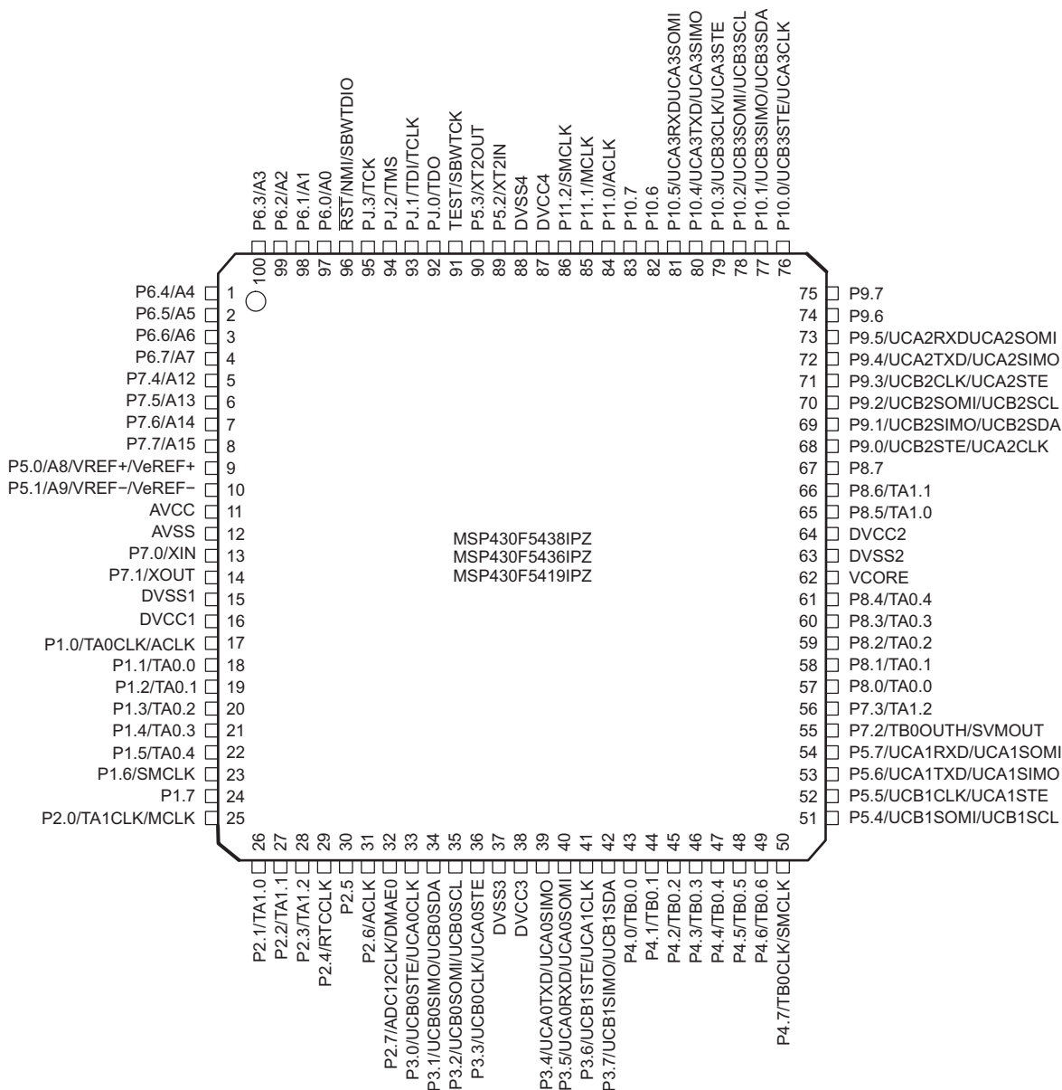
Figure 4-1. 100-Pin PZ Package (Top View) – MSP430F5438IPZ, MSP430F5436IPZ, MSP430F5419IPZ
