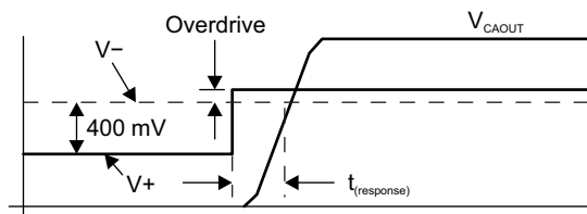
Figure 5-9. Overdrive Definition
