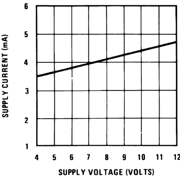
图 9-4. Supply Current vs Supply Voltage
