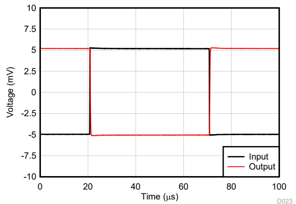
G = -1 , R_L = \text{开路} , R_{FB} = 10\text{k}\Omega
