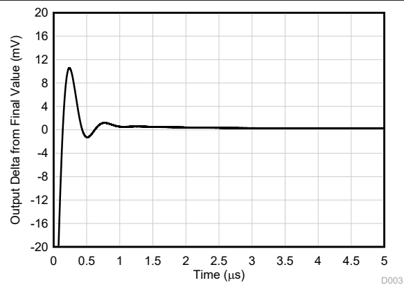
G = 1 , R_L = \text{开路}
