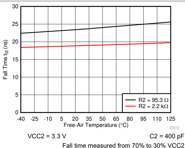
图 6-6. Side 2: Output Fall Time vs Free-Air Temperature
