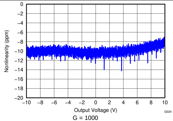
Figure 40. Gain Nonlinearity
