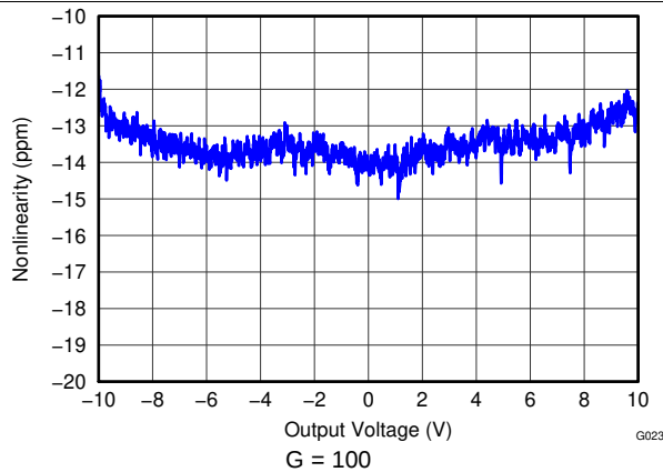
Figure 39. Gain Nonlinearity
