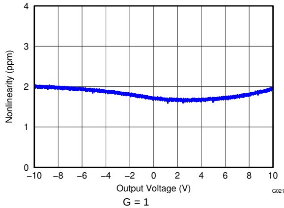
Figure 37. Gain Nonlinearity
