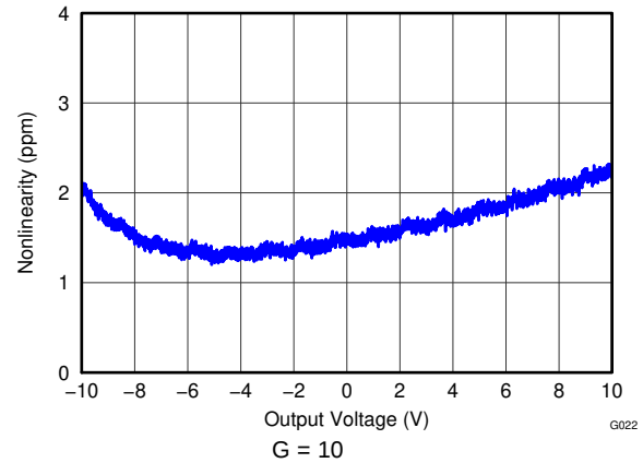
Figure 38. Gain Nonlinearity
