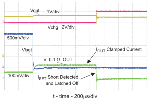
图 10-4. ISET Shorted During Normal Operation
