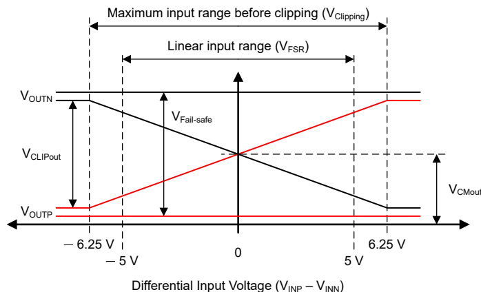
图 7-2. Output Behavior of the AMC1350
