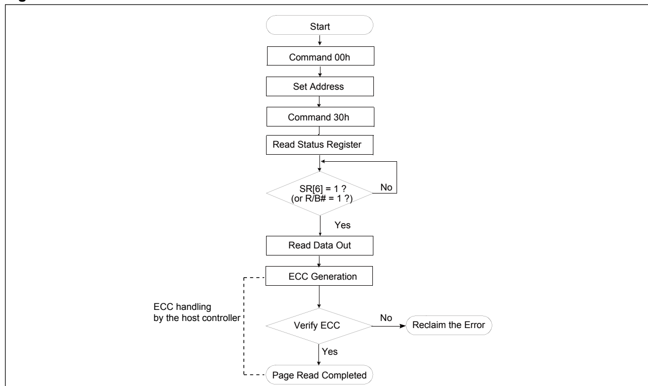
Figure 51. Read Flow Chart
