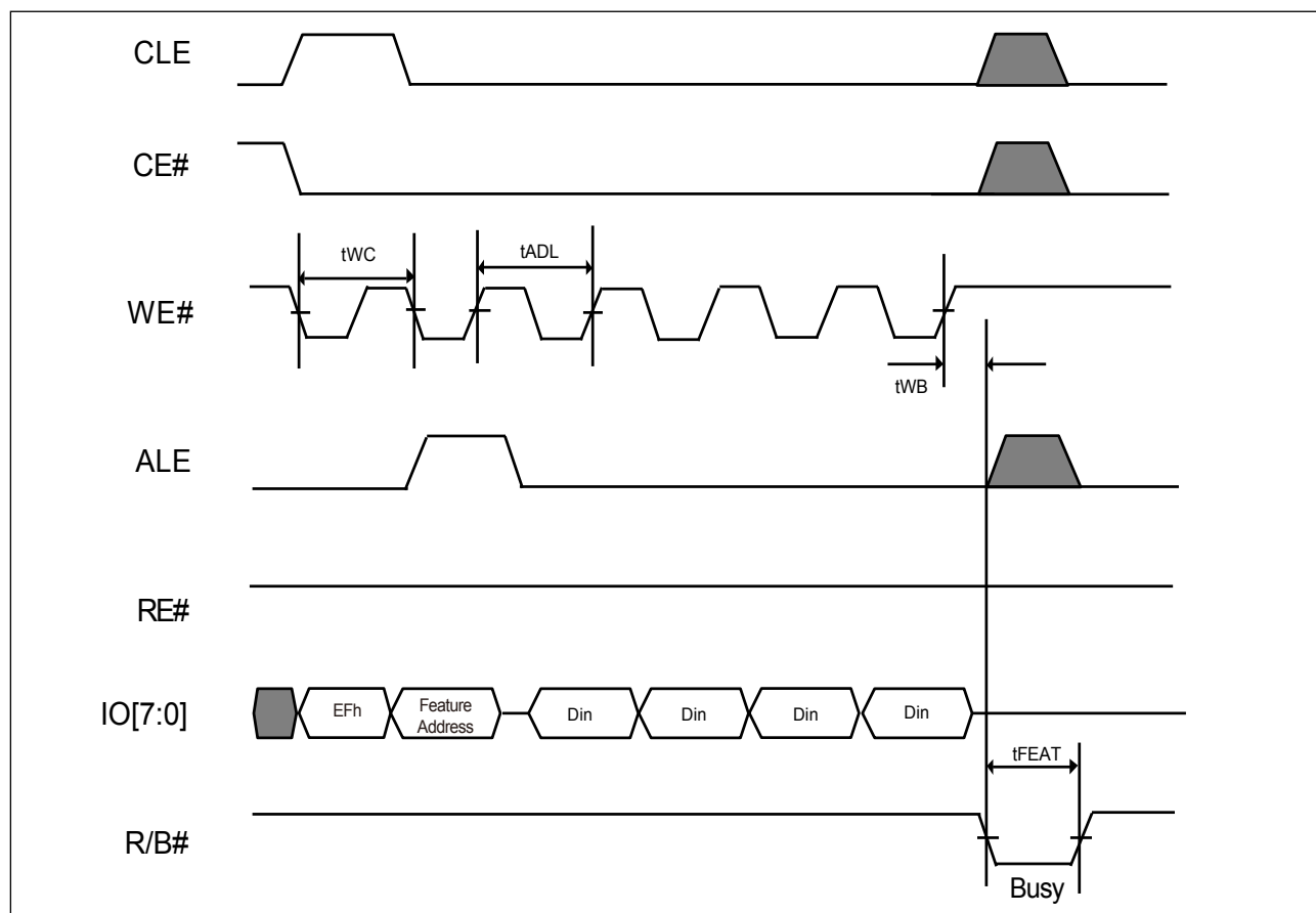
Figure 27. AC Waveforms for Set Feature (ONFI) Operation
