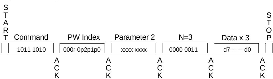
Figure 8-18. Verify Password
